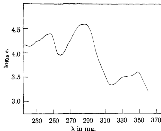
Fig. 1.—Ultraviolet absorption spectrum of 1,4,8-trimethylazulene.
